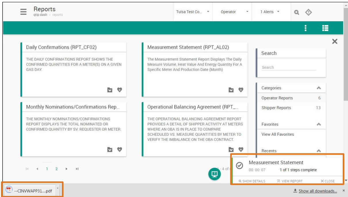
Figure 10: Report icon
