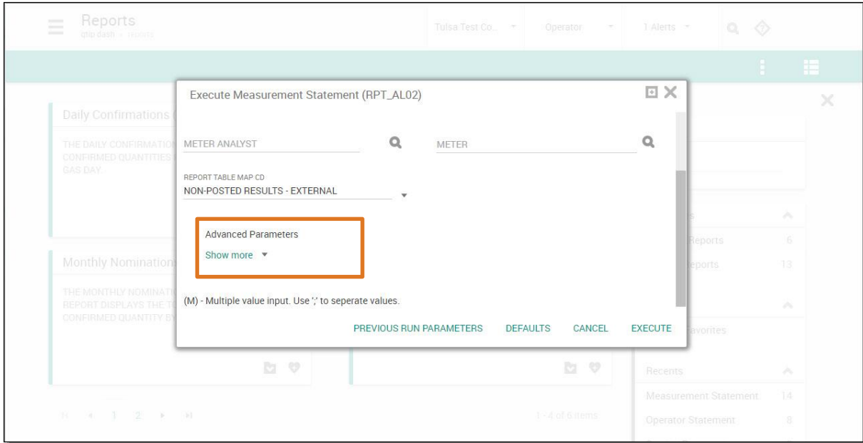
Figure 8: Advanced Parameters
