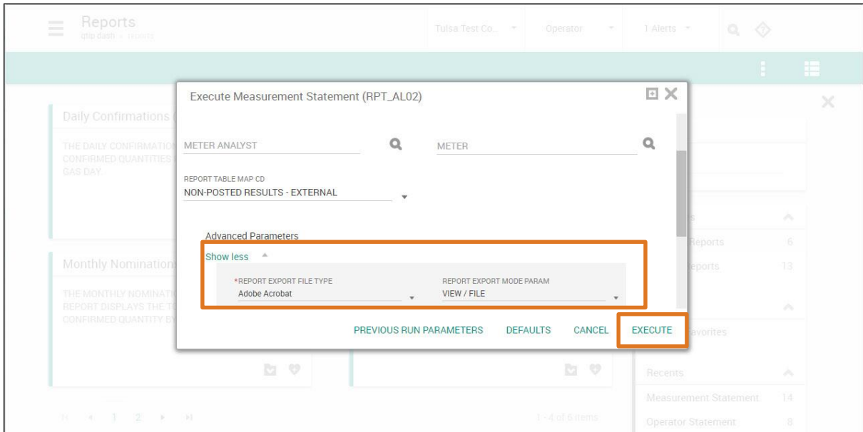
Figure 9: Execute
