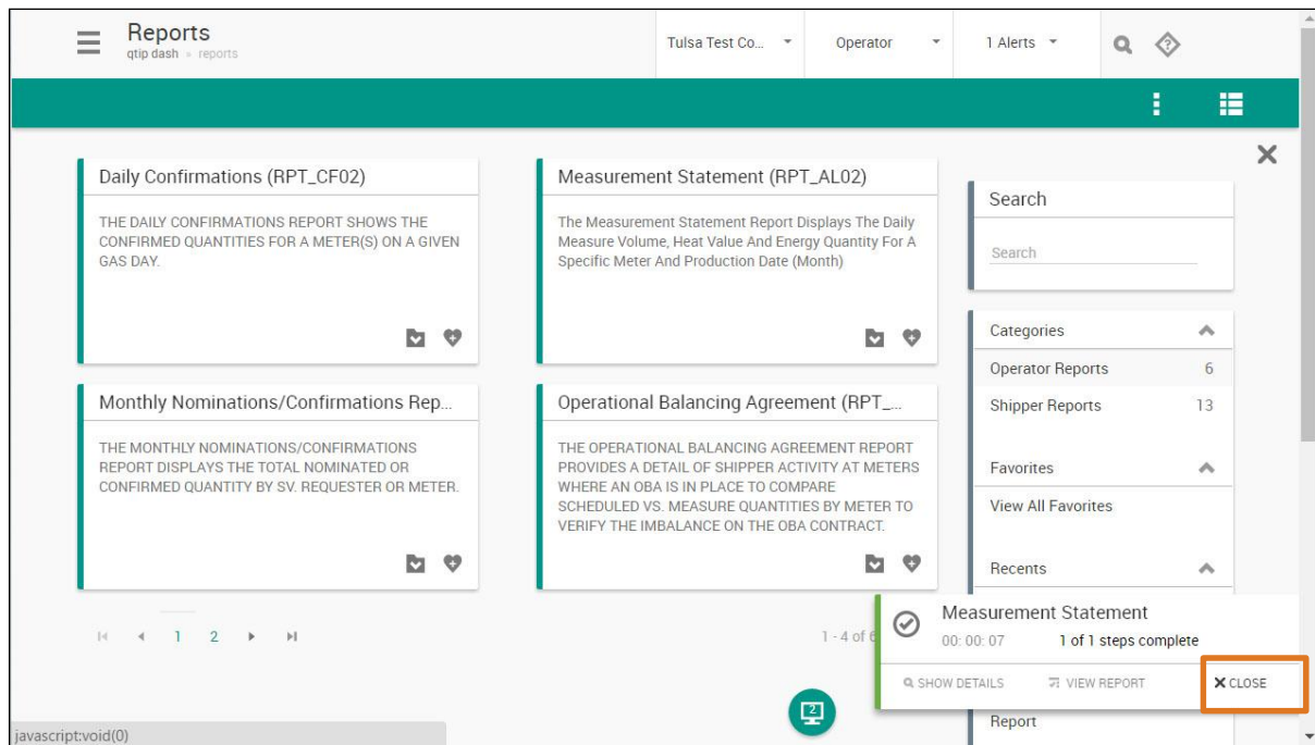
Figure 12: Close
